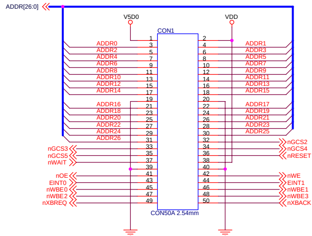
baseboard_con12
